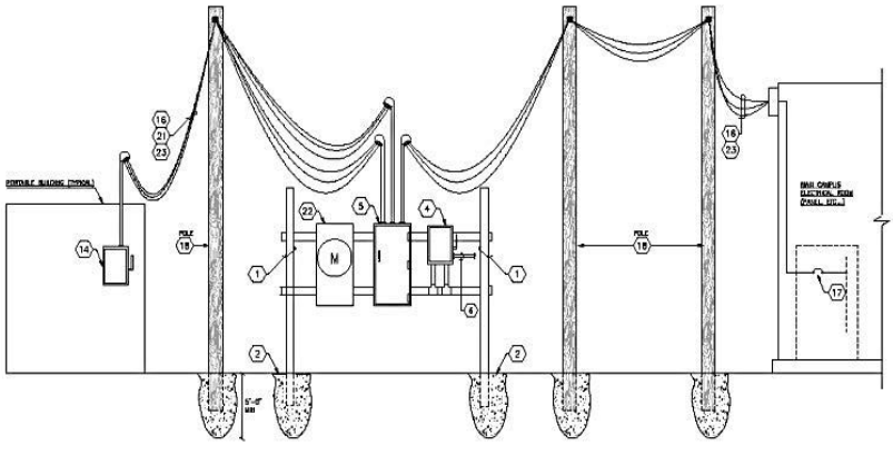
PORTABLE BUILDING POWER RISER DIAGRAM (OVERHEAD) (SCHOOL ELECTRICAL DISTRIBUTION SYSTEM) NO SCALE
