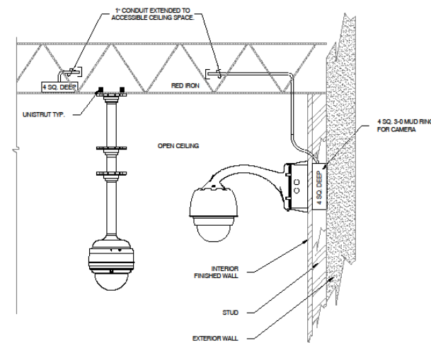
INTERIOR OPEN CEILING WALL & CEILING MOUNT ROUGH-IN NOT TO SCALE
