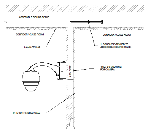
INTERIOR WALL MOUNT ROUGH-IN NOT TO SCALE
