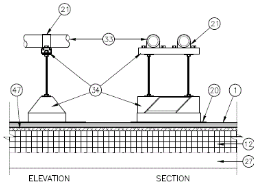
A1 TYPICAL PIPE SUPPORT ON ROOF 1 1/2" = 1'-0" 1802450101
